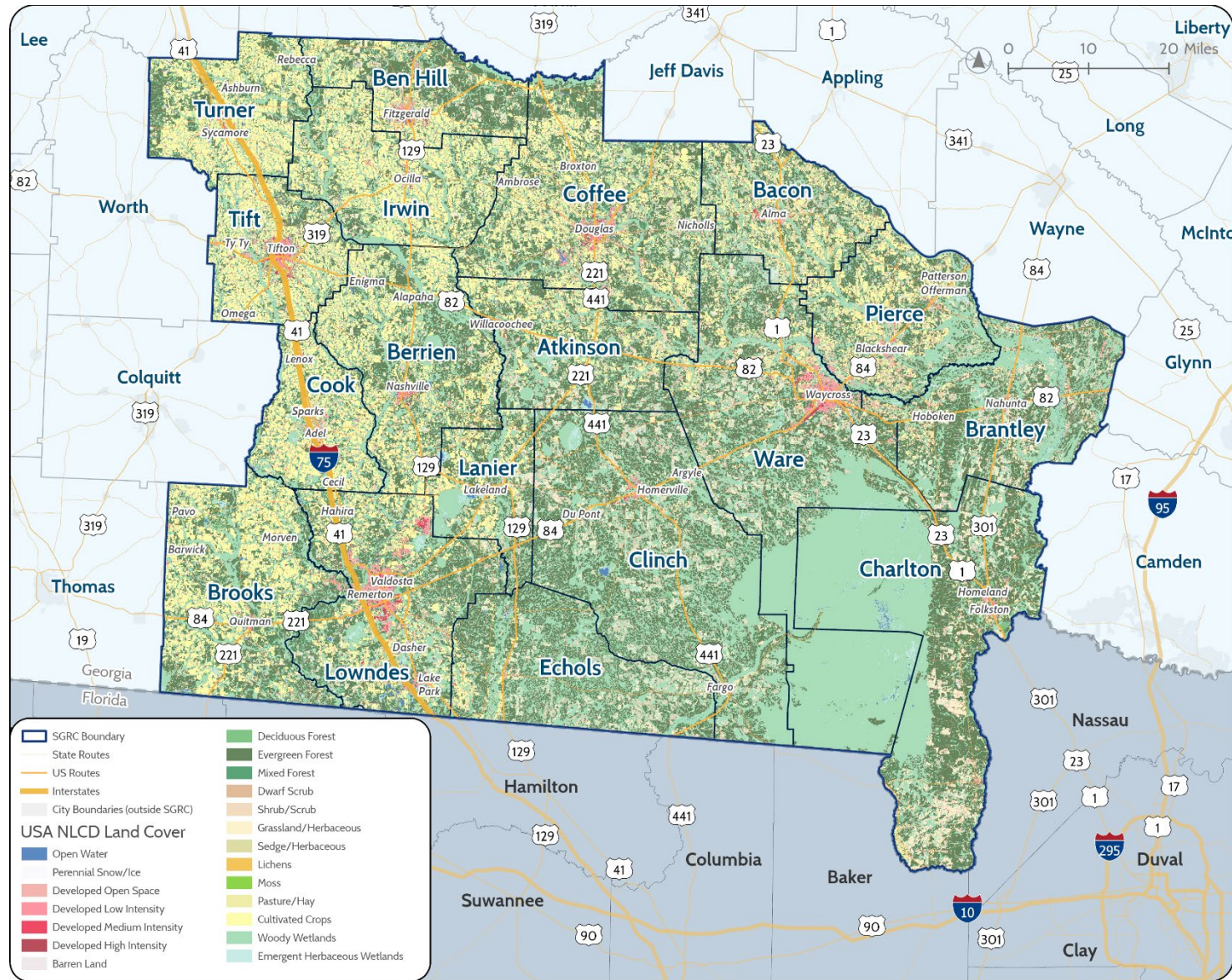
Figure 32: Land Cover
